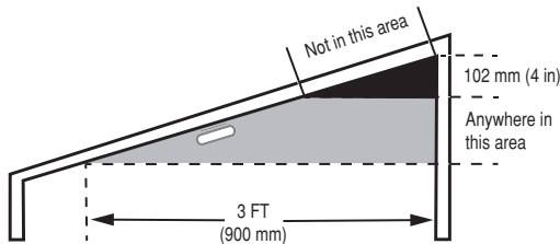
Figure 7. Example of proper mounting for Detectors with sloped ceilings
